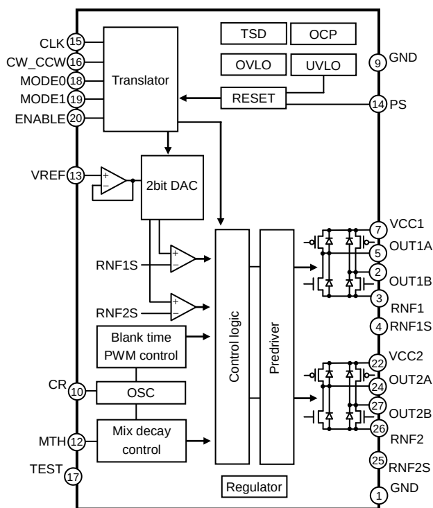
Figure.3 BD63524EFV Block Diagram
